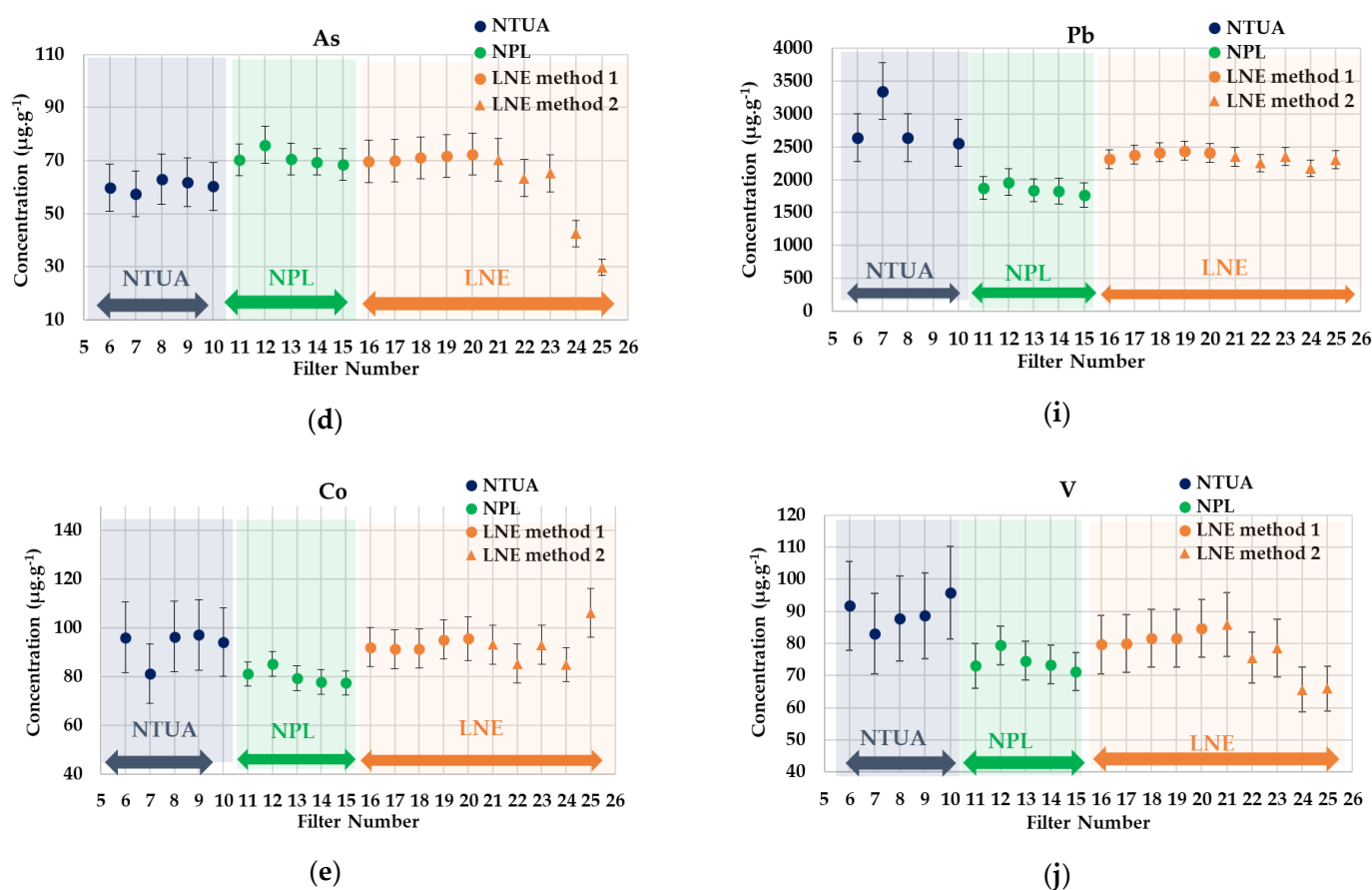
Figure 4. ICP-MS intercomparison results for PM_{2.5} -loaded filters. (a) Cr, (b) Fe, (c) Cu, (d) As, (e) Co, (f) Mn, (g) Ni, (h) Zn, (i) Pb and (j) V.
